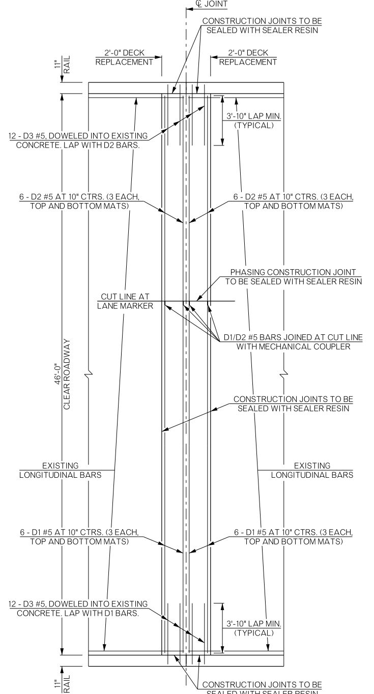
DETAIL OF DECK REPAIR AT CONSTRUCTION JOINT
