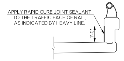
REHABILITATED CONSTRUCTION JOINT AT TRAFFIC RAIL
