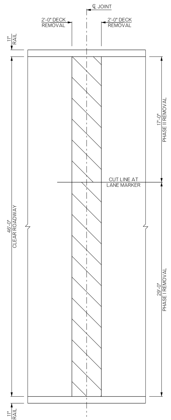
DETAIL OF DECK REMOVAL AT CONSTRUCTION JOINT
