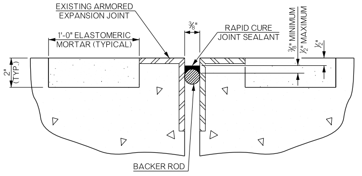
REHABILITATED EXPANSION JOINT AT ABUTMENT NO. 2
