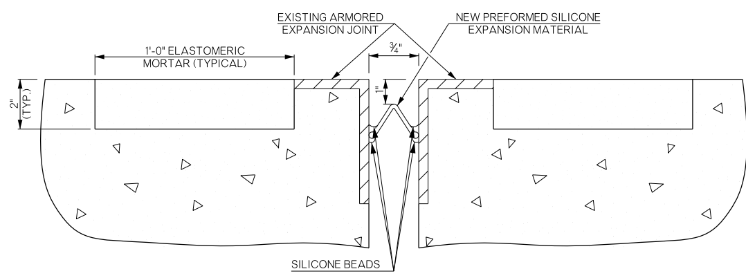
REHABILITATED EXPANSION JOINT AT ABUTMENT NO. 1
